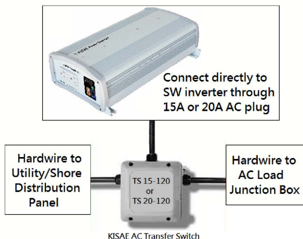
TS 15-120 and TS 20-120 Wiring Block Diagram
