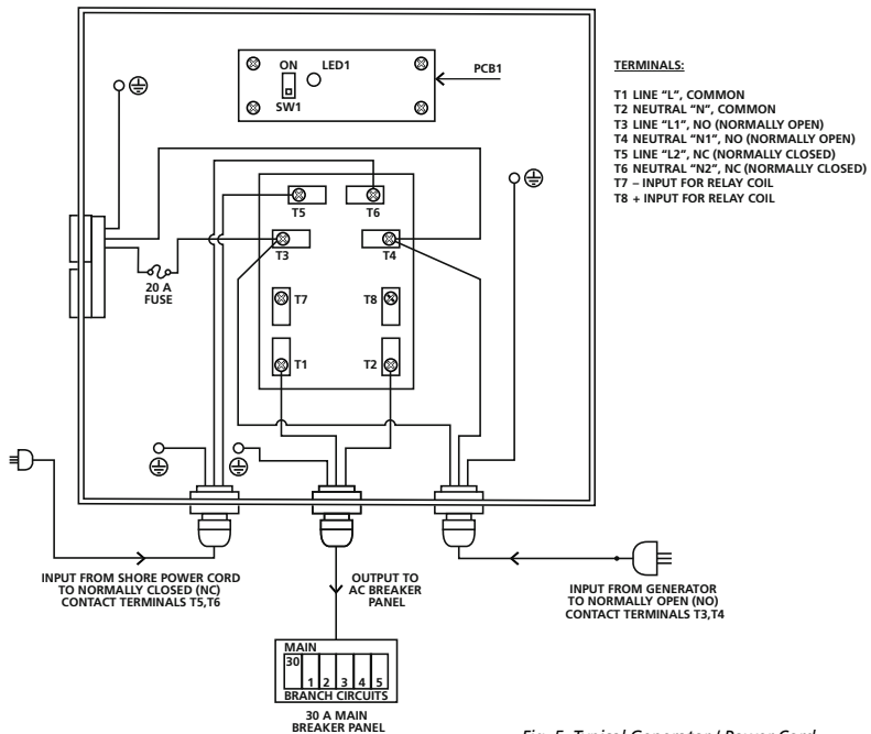
Fig. 5 Typical Generator / Power Cord
