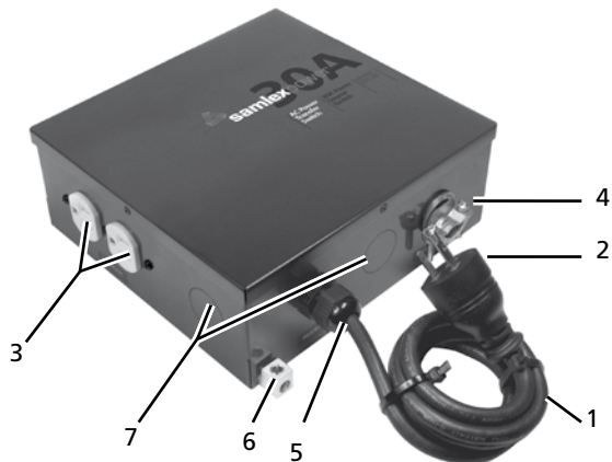
Fig. 1 External view and layout
