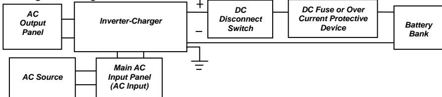
Wiring block diagram of the Inverter-Charger
